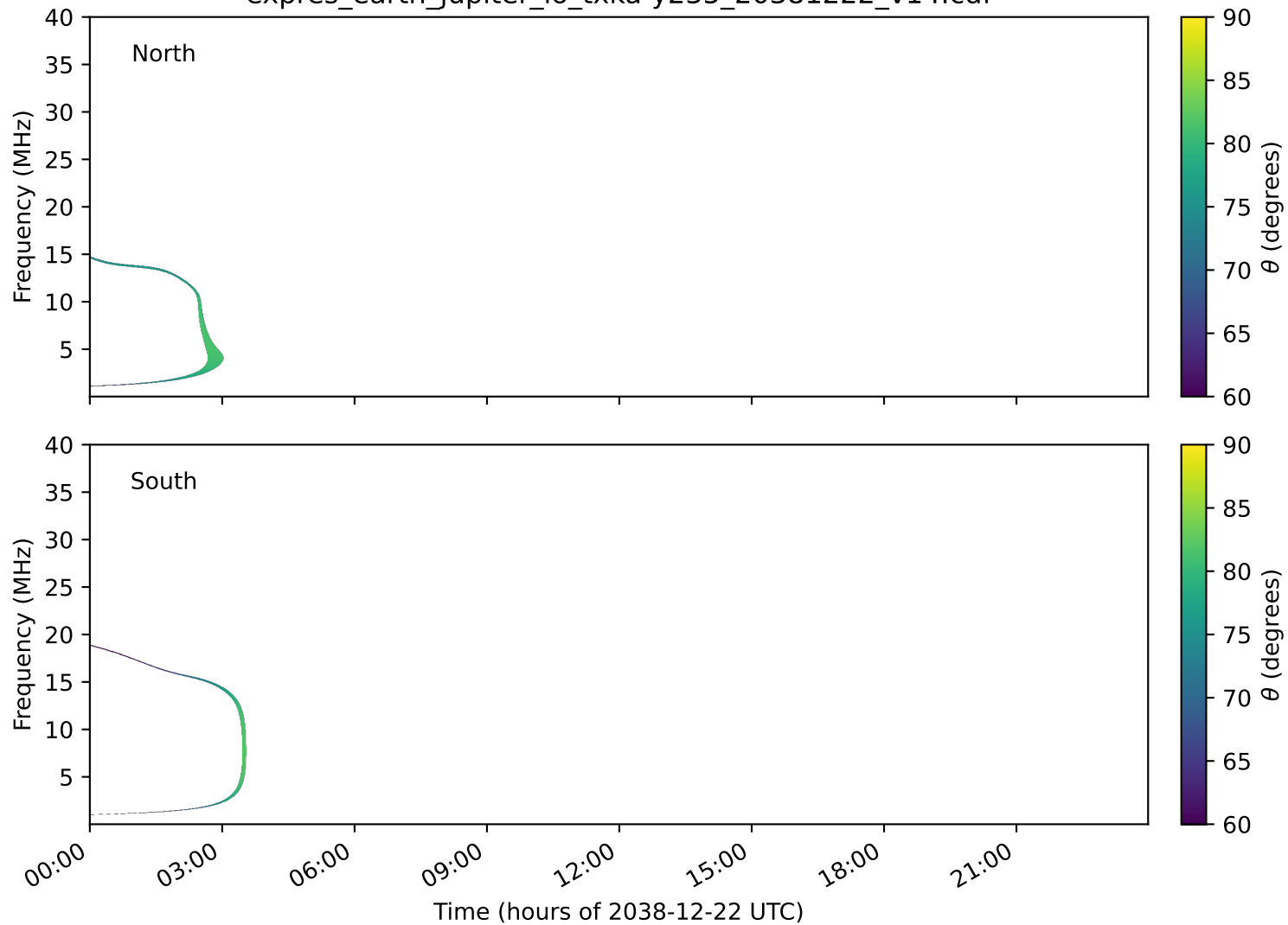
expres_earth_jupiter_io_txka-y235_20381222_v14.cdf
