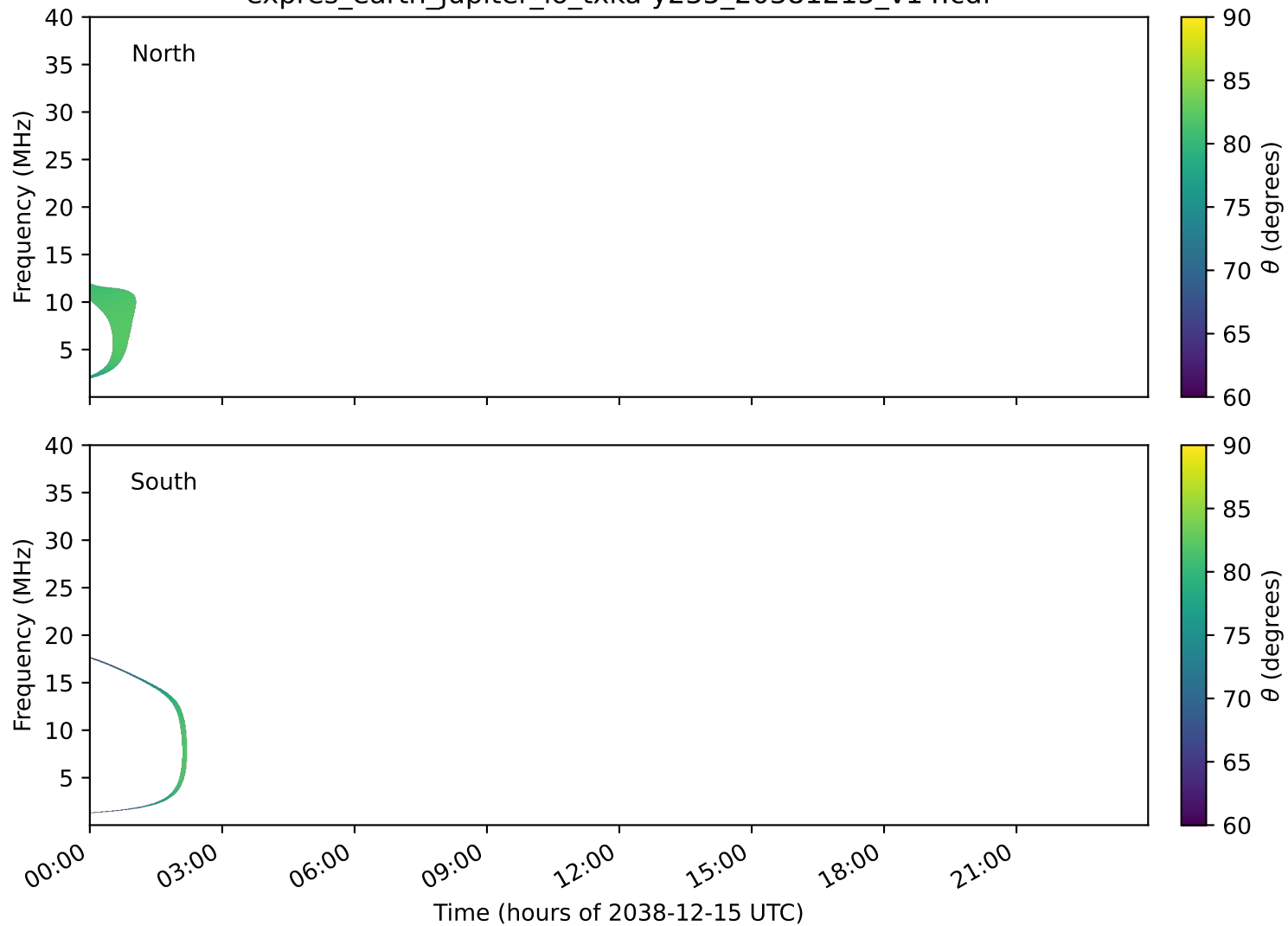
expres_earth_jupiter_io_txka-y235_20381215_v14.cdf
