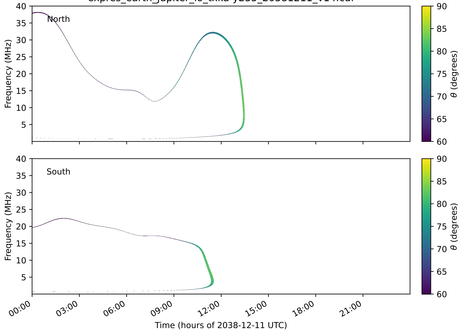
expres_earth_jupiter_io_txka-y235_20381211_v14.cdf
