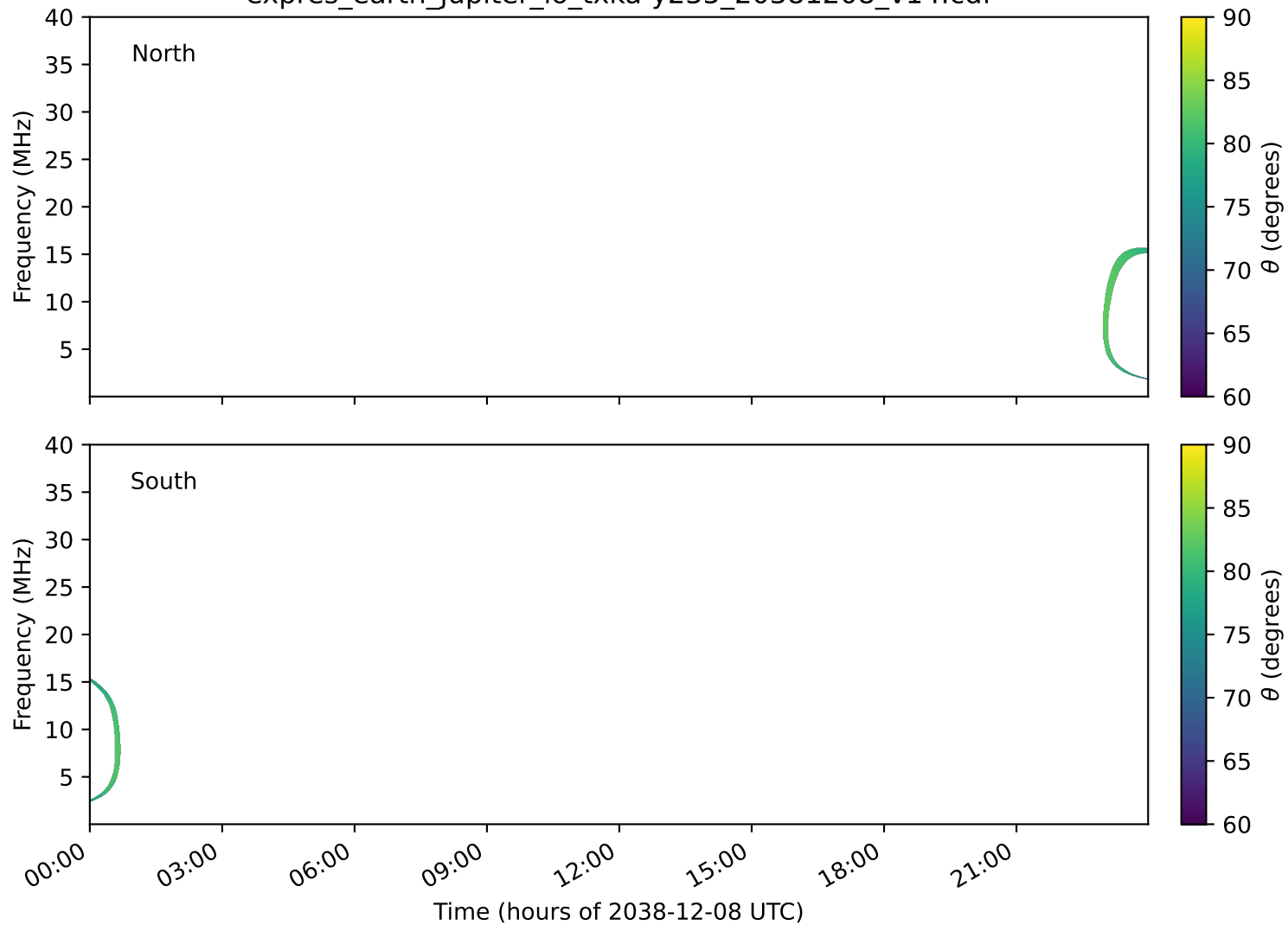
expres_earth_jupiter_io_txka-y235_20381208_v14.cdf
