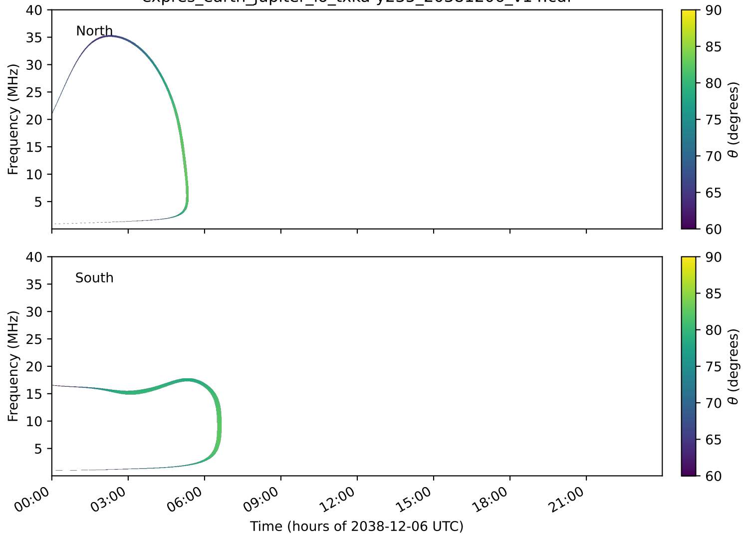
expres_earth_jupiter_io_txka-y235_20381206_v14.cdf
