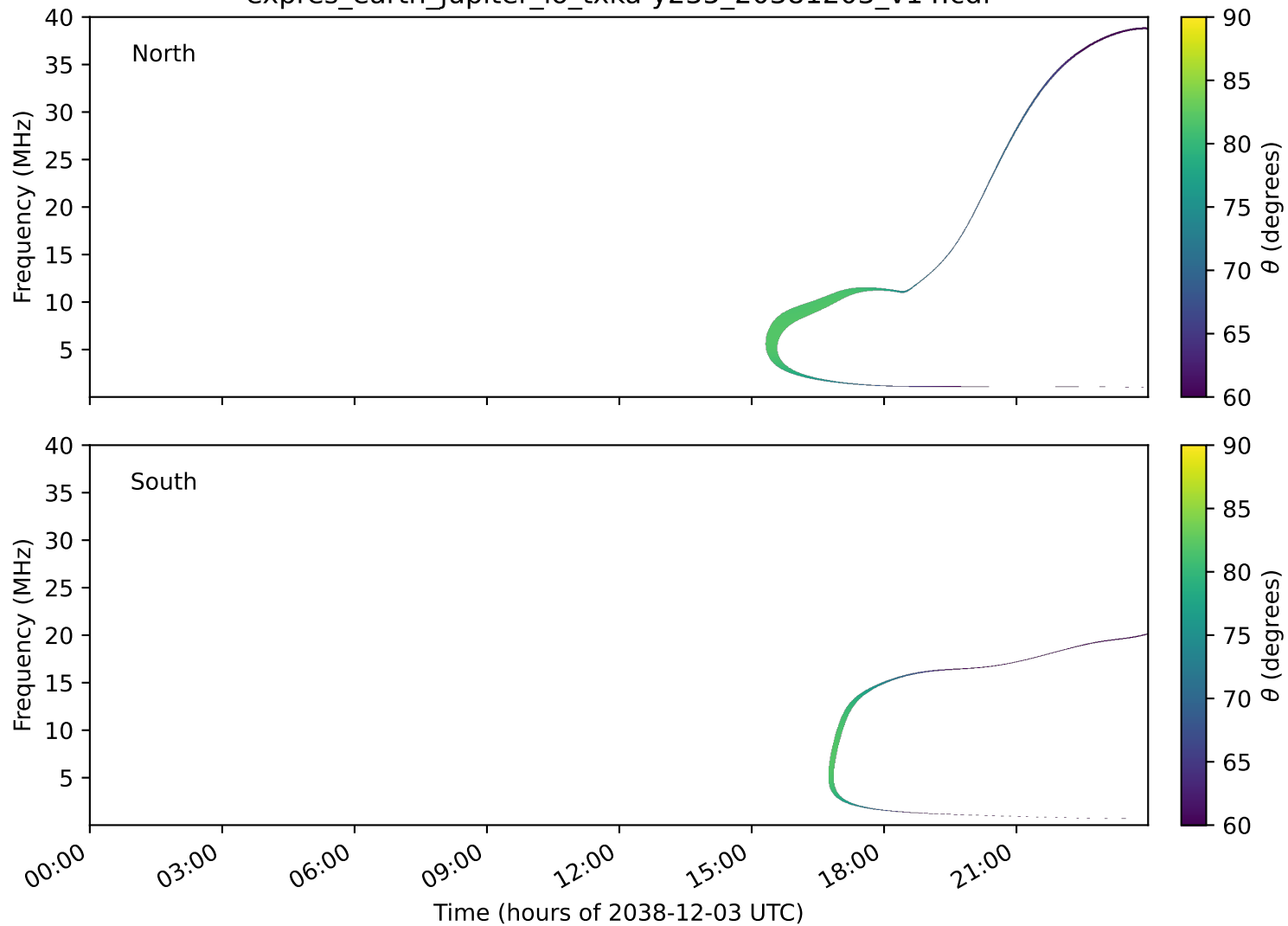
expres_earth_jupiter_io_txka-y235_20381203_v14.cdf
