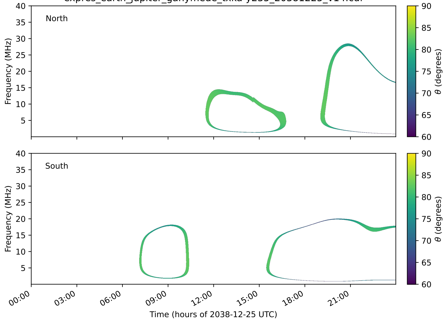
expres_earth_jupiter_ganymede_txka-y235_20381225_v14.cdf
