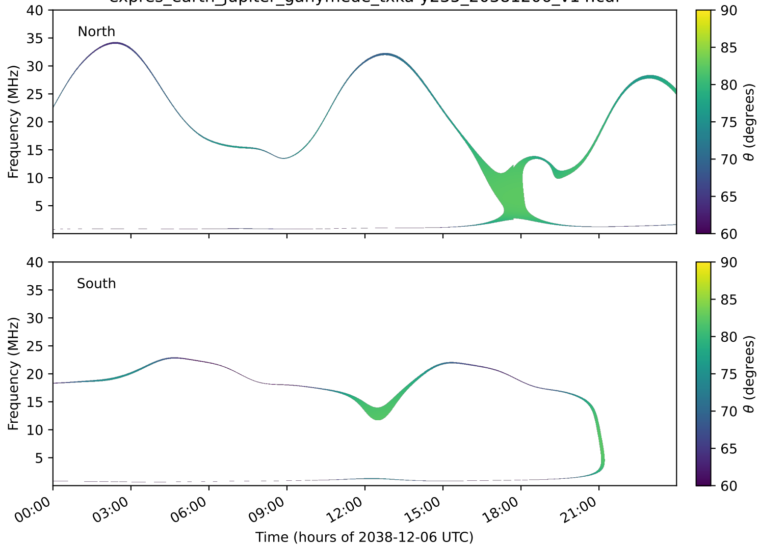
expres_earth_jupiter_ganymede_txka-y235_20381206_v14.cdf
