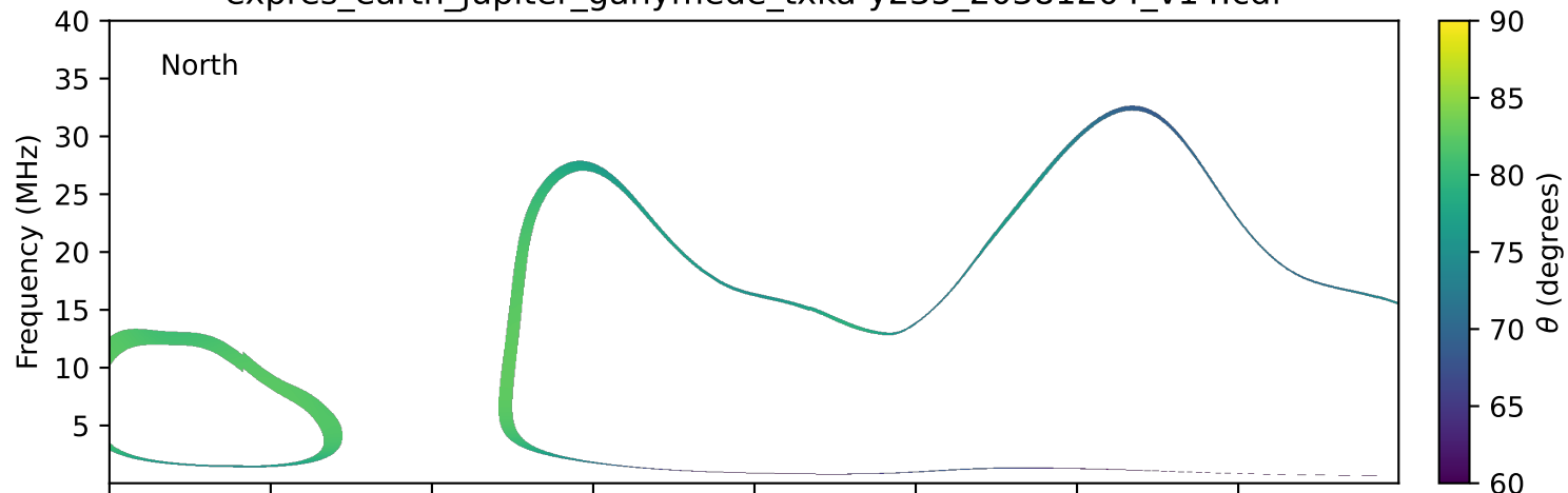
expres_earth_jupiter_ganymede_txka-y235_20381204_v14.cdf
