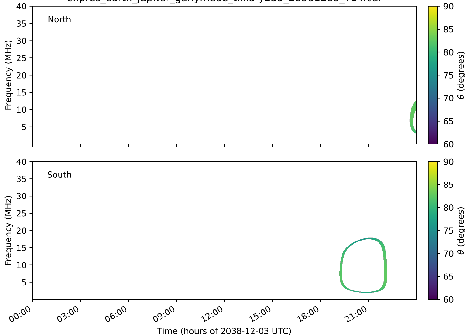
expres_earth_jupiter_ganymede_txka-y235_20381203_v14.cdf
