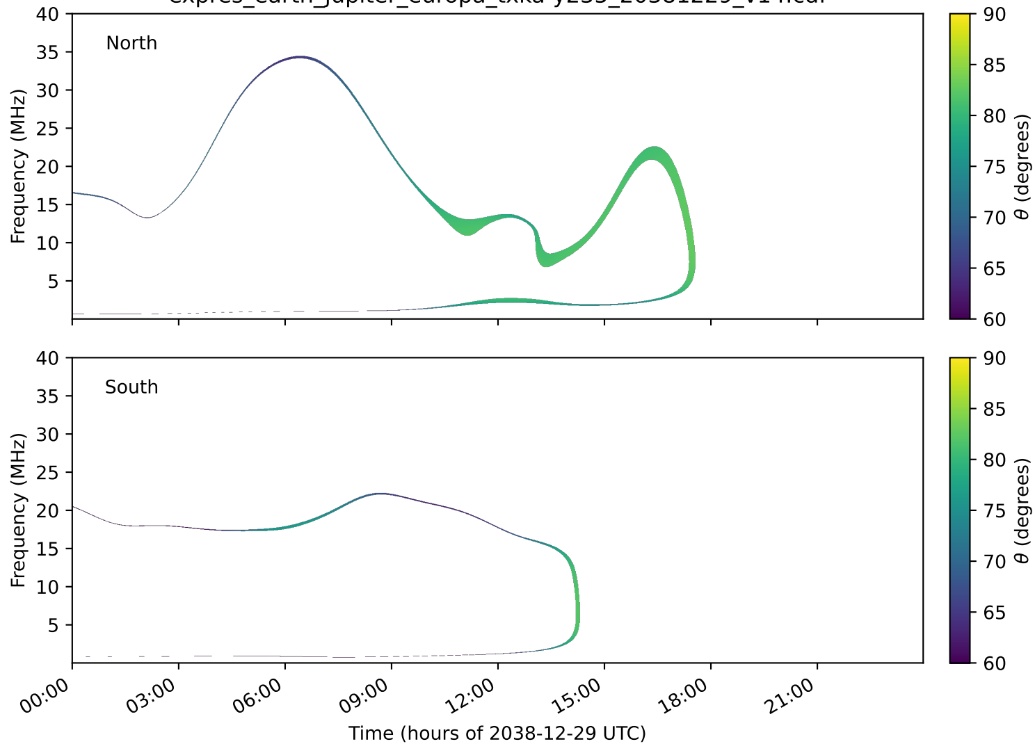
expres_earth_jupiter_europa_txka-y235_20381229_v14.cdf
