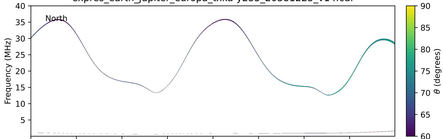
expres_earth_jupiter_europa_txka-y235_20381225_v14.cdf
