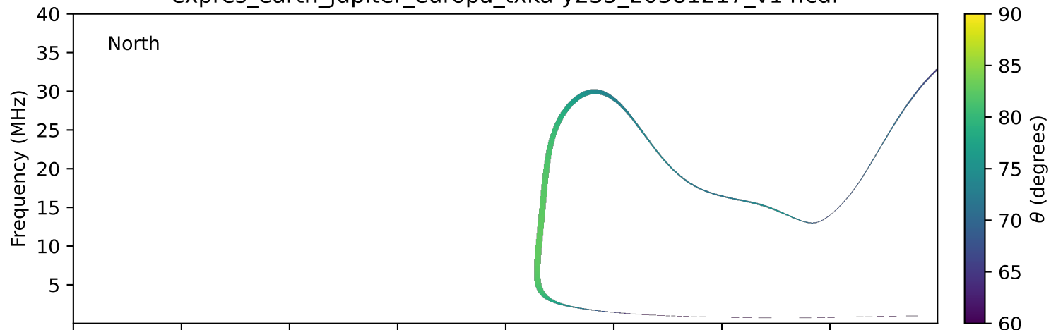
expres_earth_jupiter_europa_txka-y235_20381217_v14.cdf
