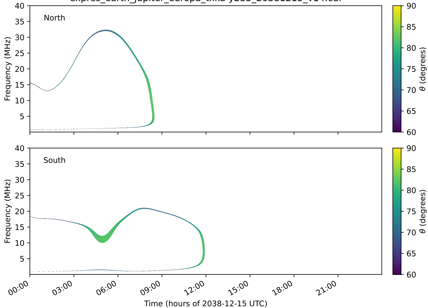
expres_earth_jupiter_europa_txka-y235_20381215_v14.cdf
