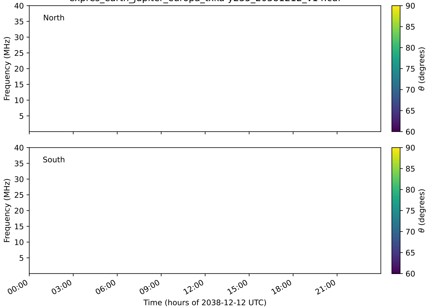
expres_earth_jupiter_europa_txka-y235_20381212_v14.cdf
