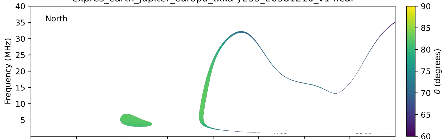
expres_earth_jupiter_europa_txka-y235_20381210_v14.cdf
