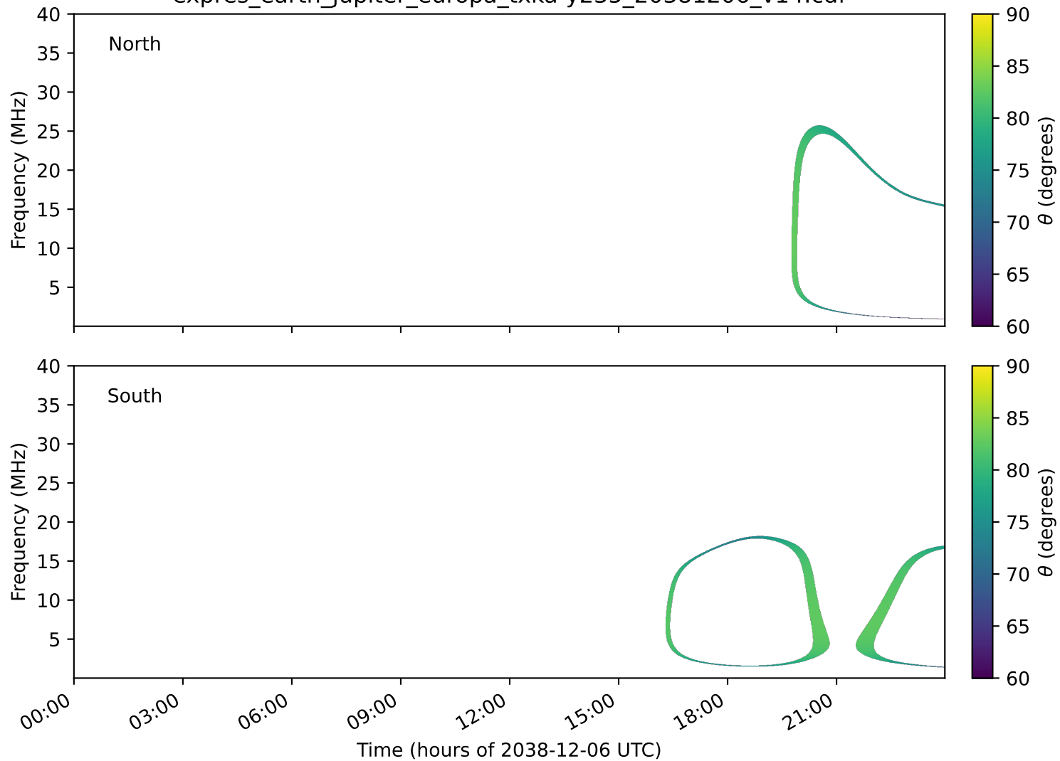
expres_earth_jupiter_europa_txka-y235_20381206_v14.cdf
