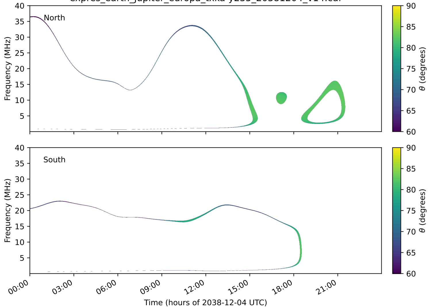
expres_earth_jupiter_europa_txka-y235_20381204_v14.cdf
