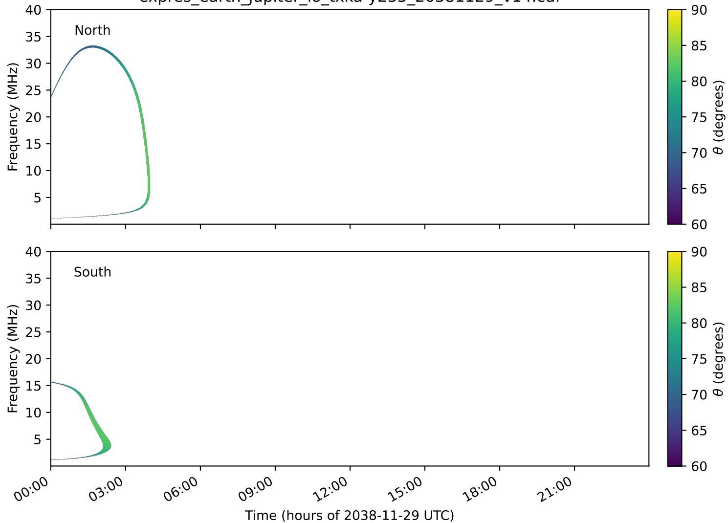
expres_earth_jupiter_io_txka-y235_20381129_v14.cdf
