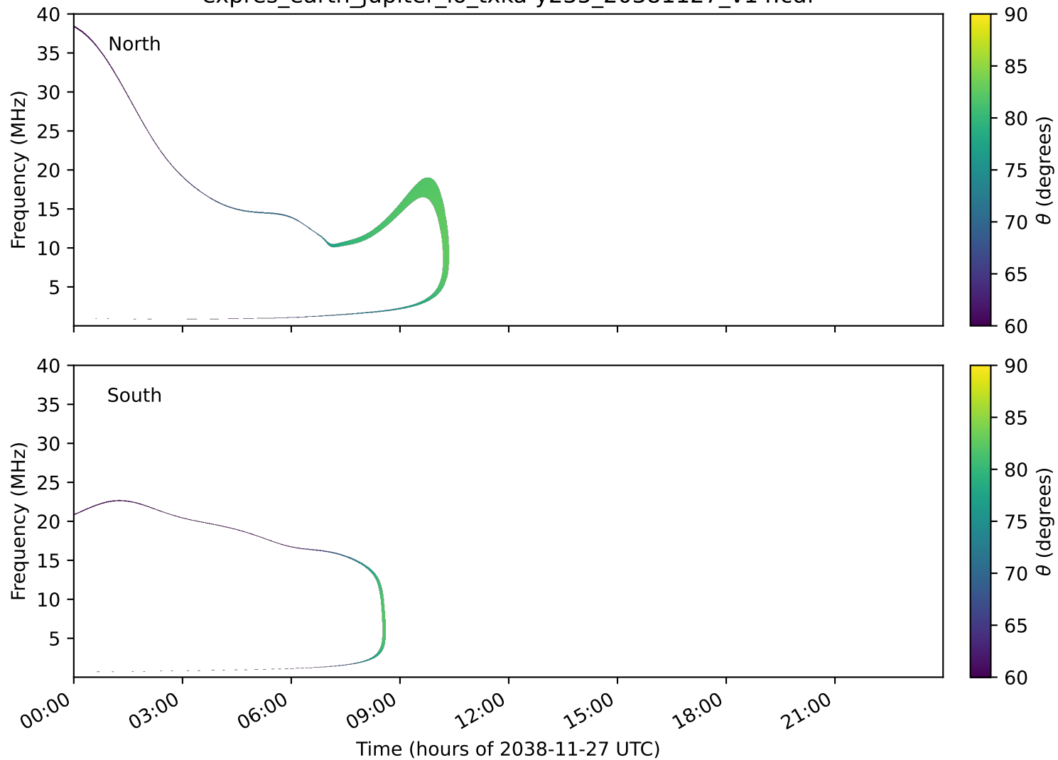
expres_earth_jupiter_io_txka-y235_20381127_v14.cdf
