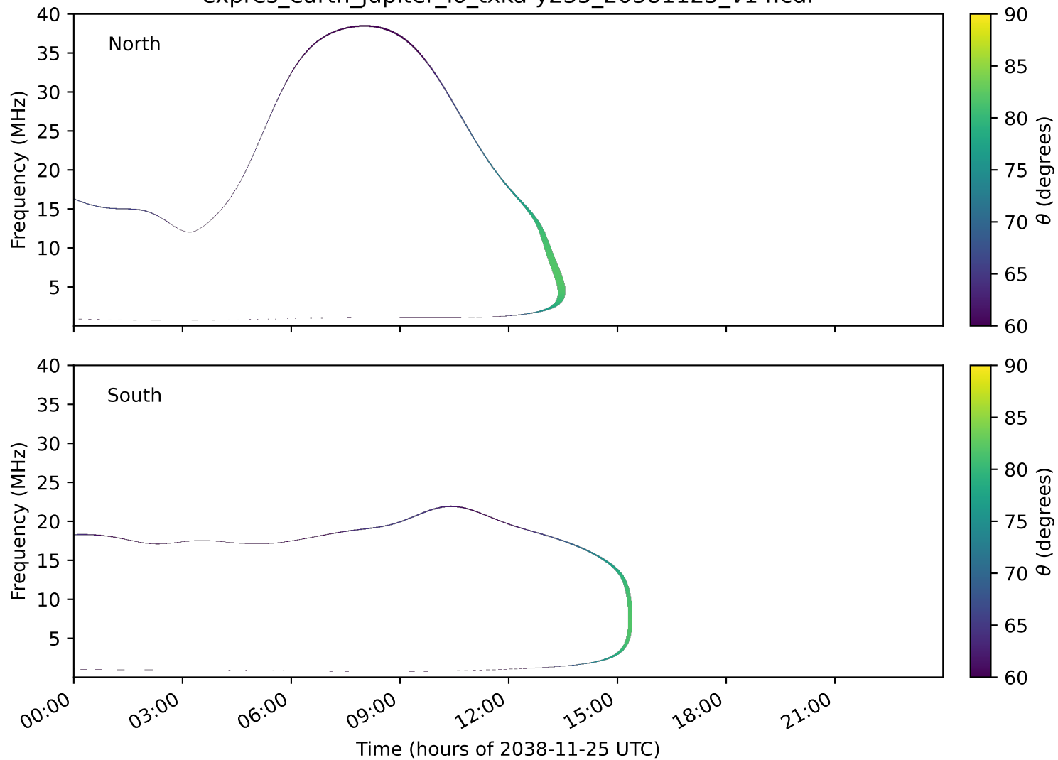
expres_earth_jupiter_io_txka-y235_20381125_v14.cdf
