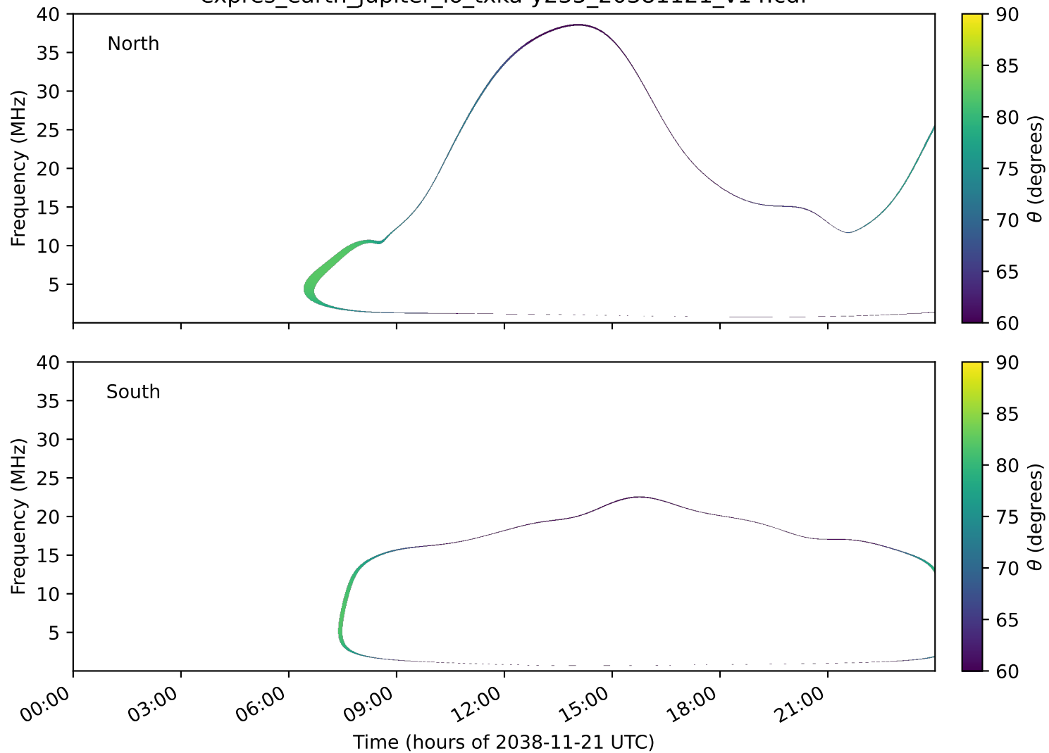
expres_earth_jupiter_io_txka-y235_20381121_v14.cdf
