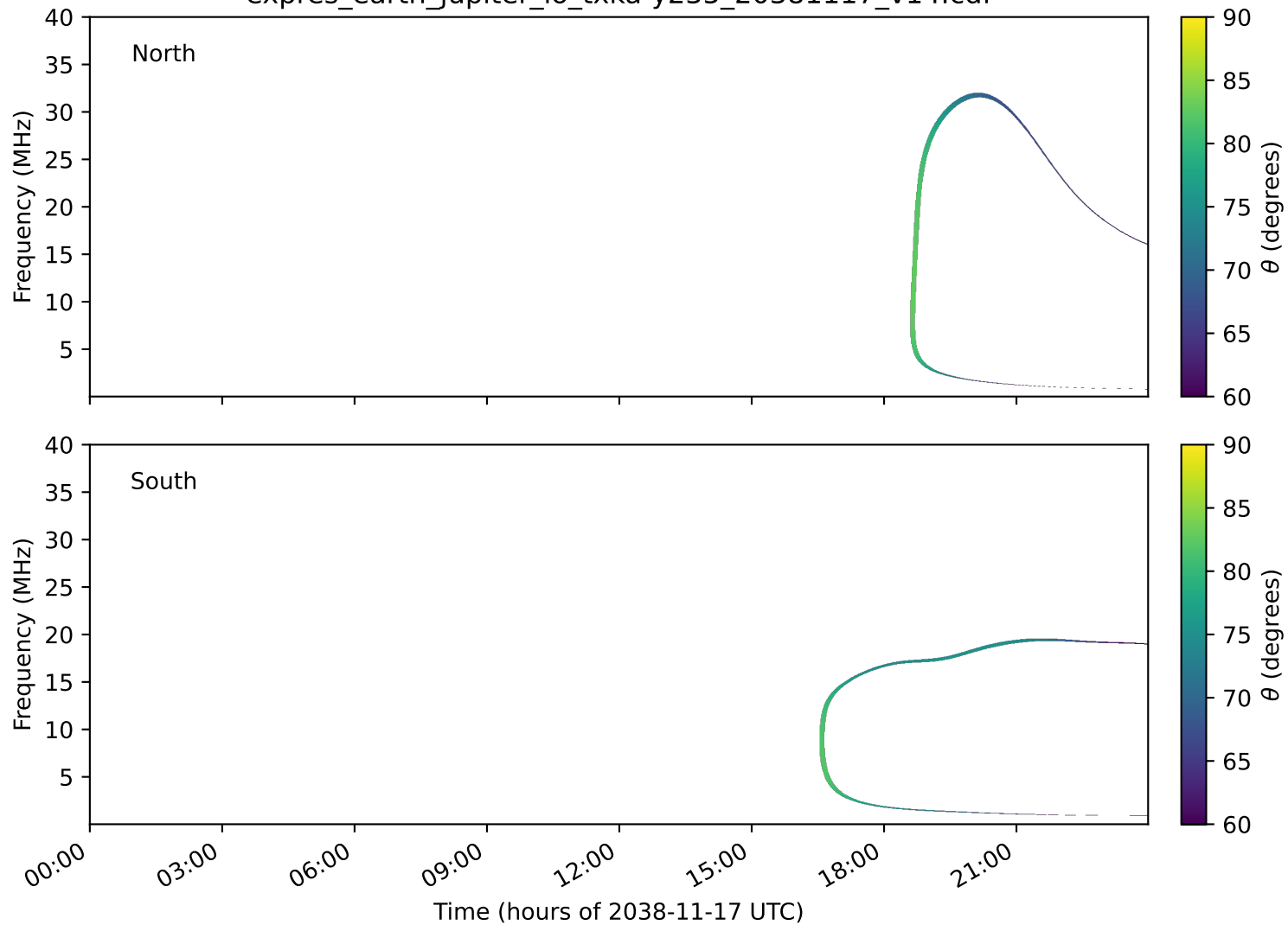
expres_earth_jupiter_io_txka-y235_20381117_v14.cdf
