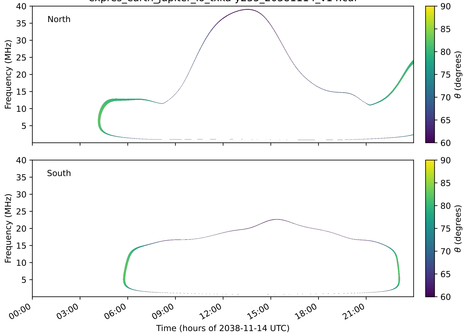
expres_earth_jupiter_io_txka-y235_20381114_v14.cdf
