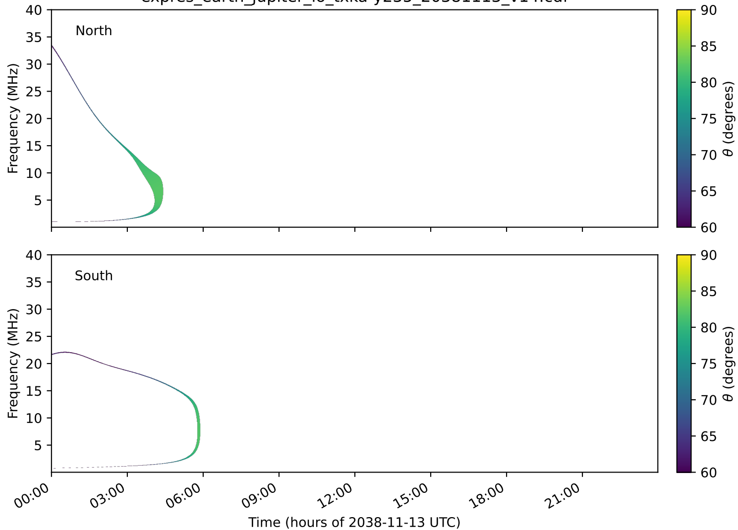
expres_earth_jupiter_io_txka-y235_20381113_v14.cdf
