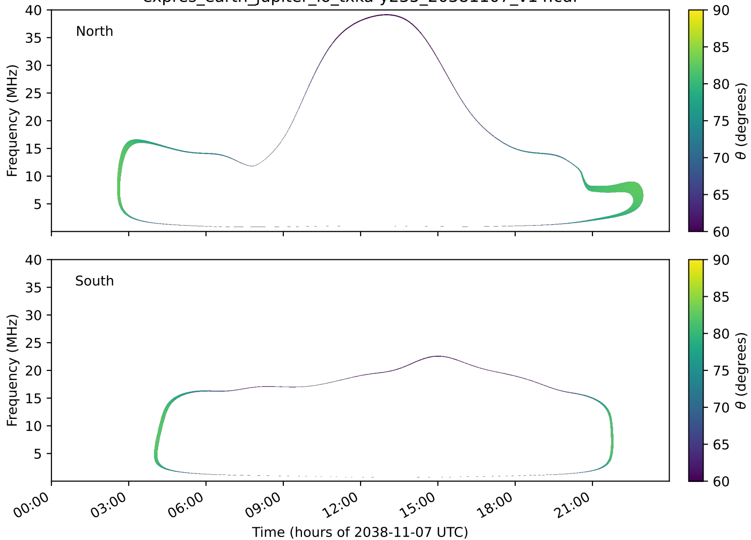
expres_earth_jupiter_io_txka-y235_20381107_v14.cdf
