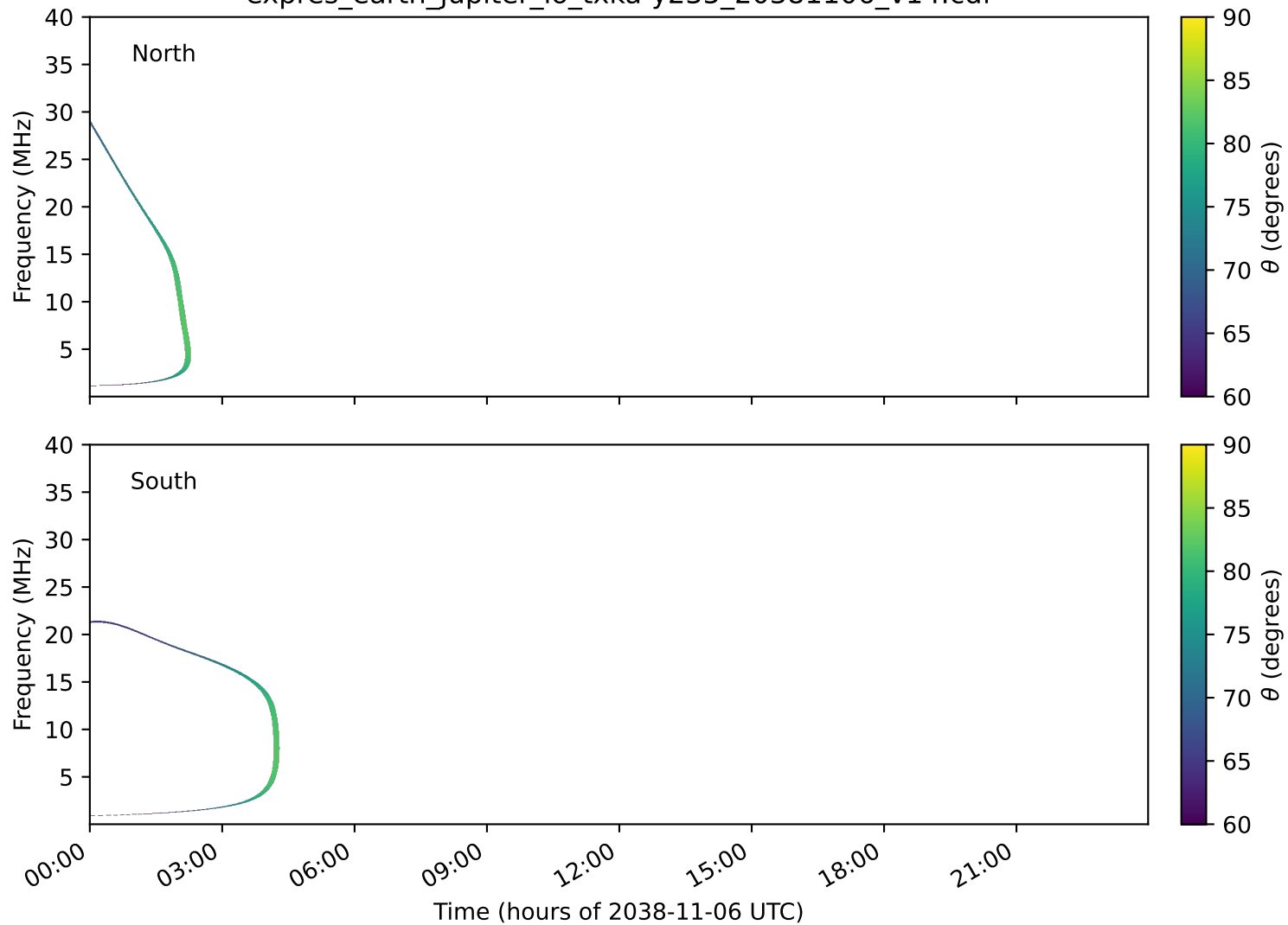
expres_earth_jupiter_io_txka-y235_20381106_v14.cdf
