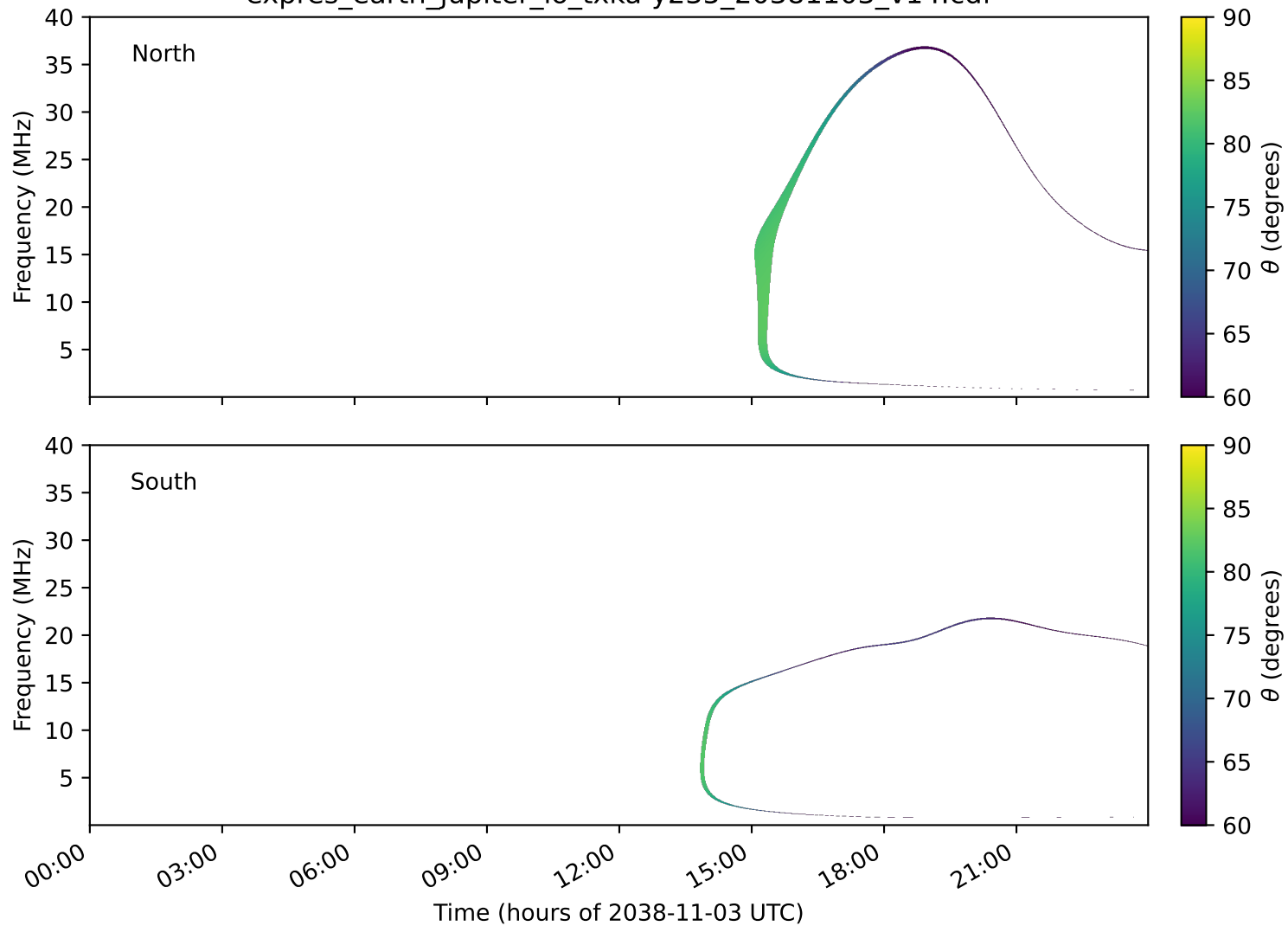
expres_earth_jupiter_io_txka-y235_20381103_v14.cdf
