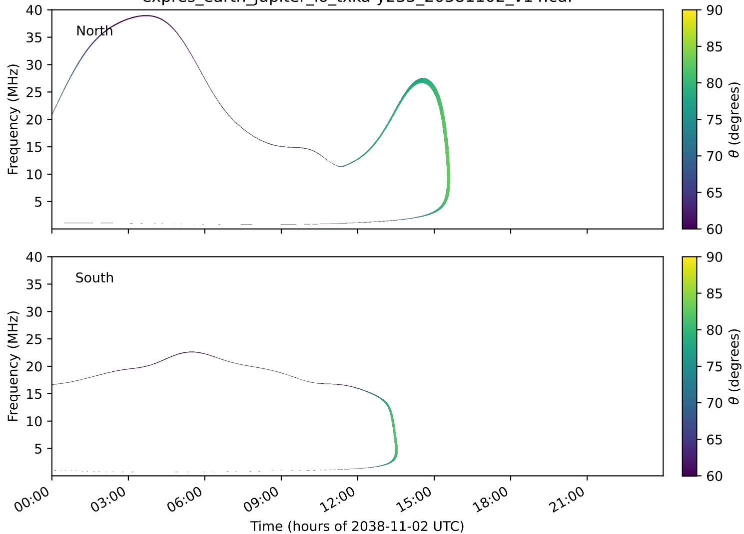
expres_earth_jupiter_io_txka-y235_20381102_v14.cdf
