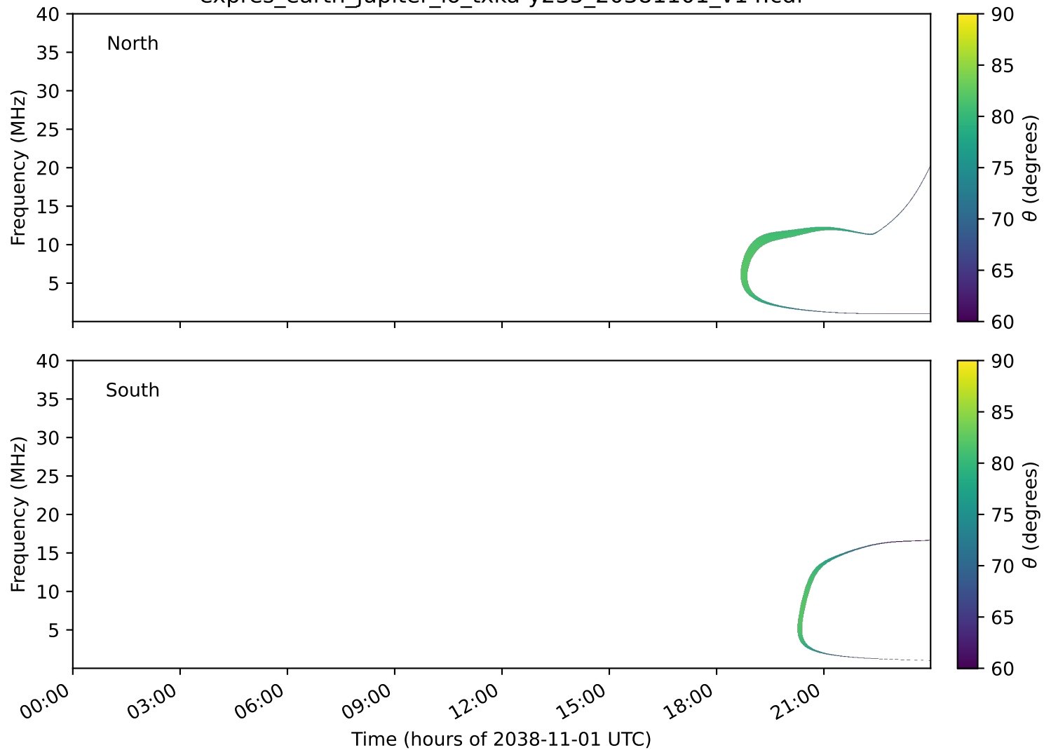
expres_earth_jupiter_io_txka-y235_20381101_v14.cdf
