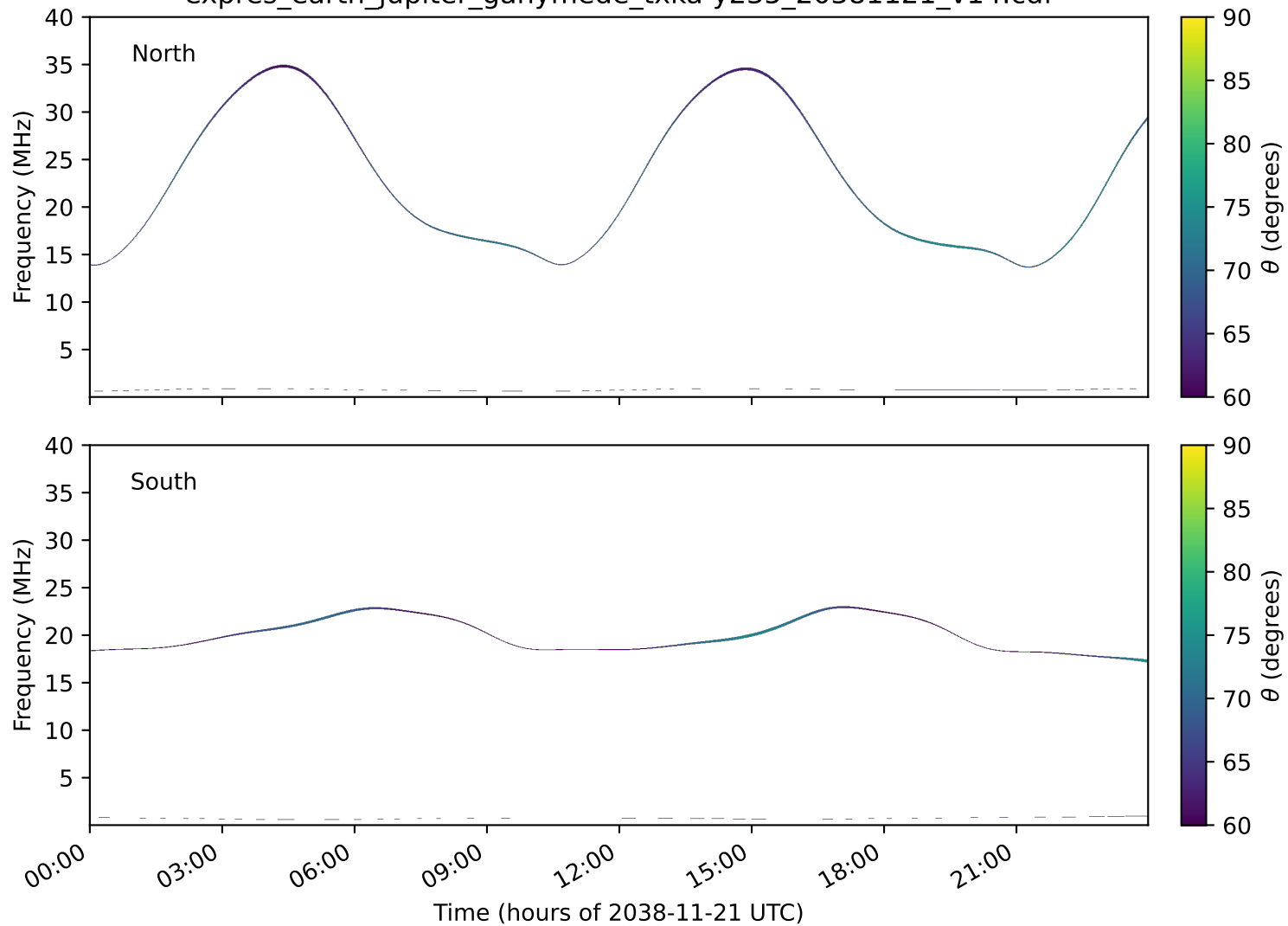
expres_earth_jupiter_ganymede_txka-y235_20381121_v14.cdf
