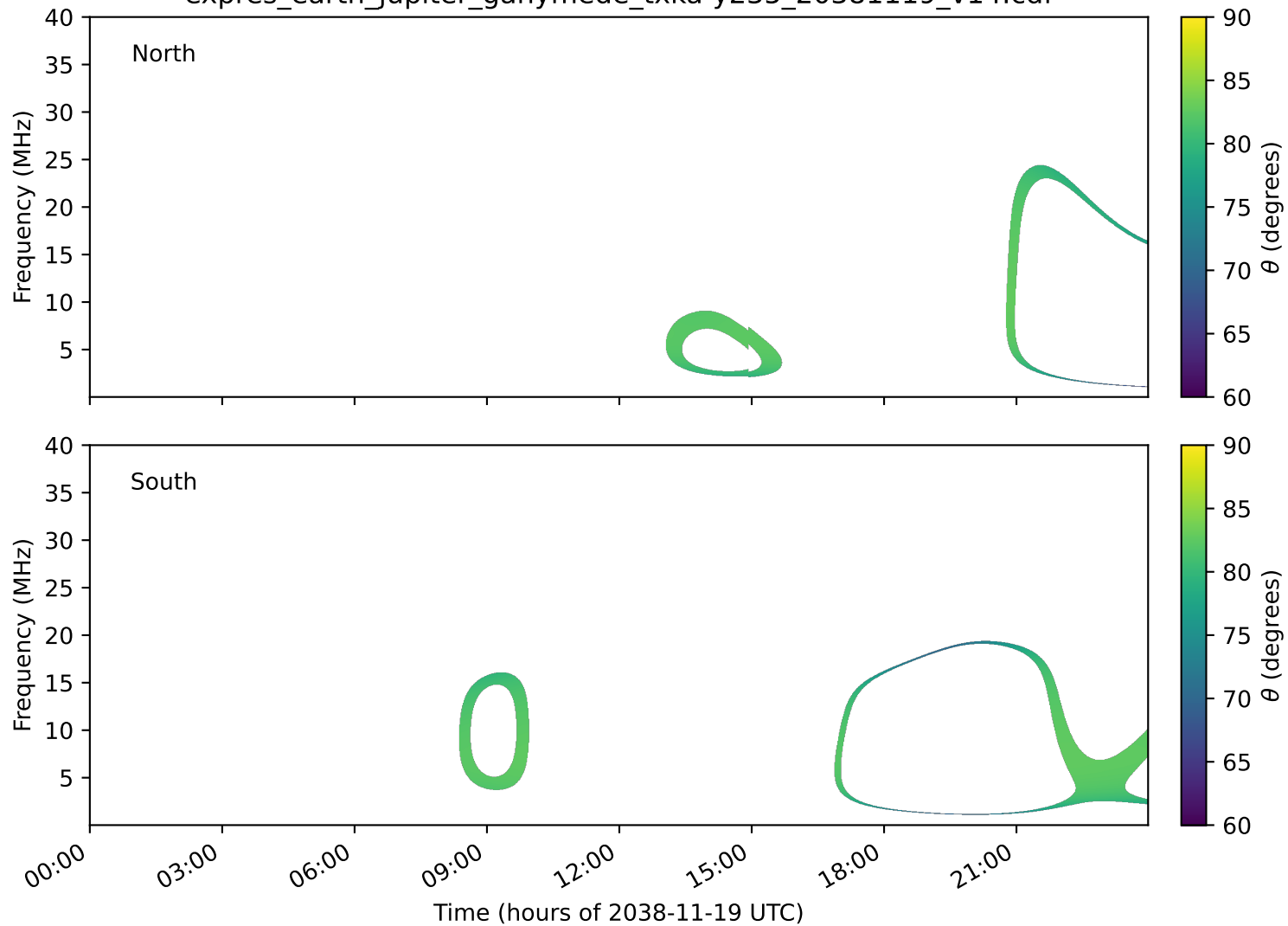
expres_earth_jupiter_ganymede_txka-y235_20381119_v14.cdf
