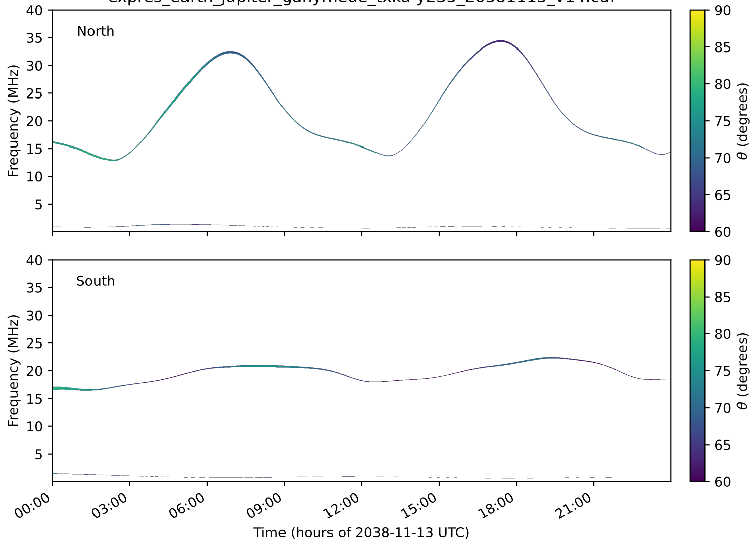
expres_earth_jupiter_ganymede_txka-y235_20381113_v14.cdf
