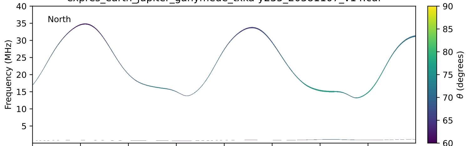
expres_earth_jupiter_ganymede_txka-y235_20381107_v14.cdf
