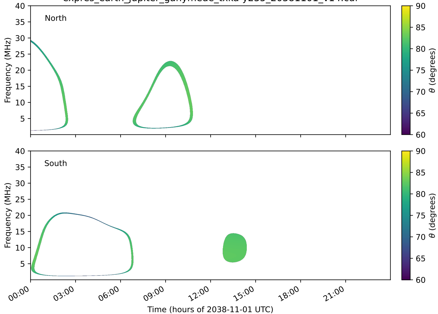
expres_earth_jupiter_ganymede_txka-y235_20381101_v14.cdf
