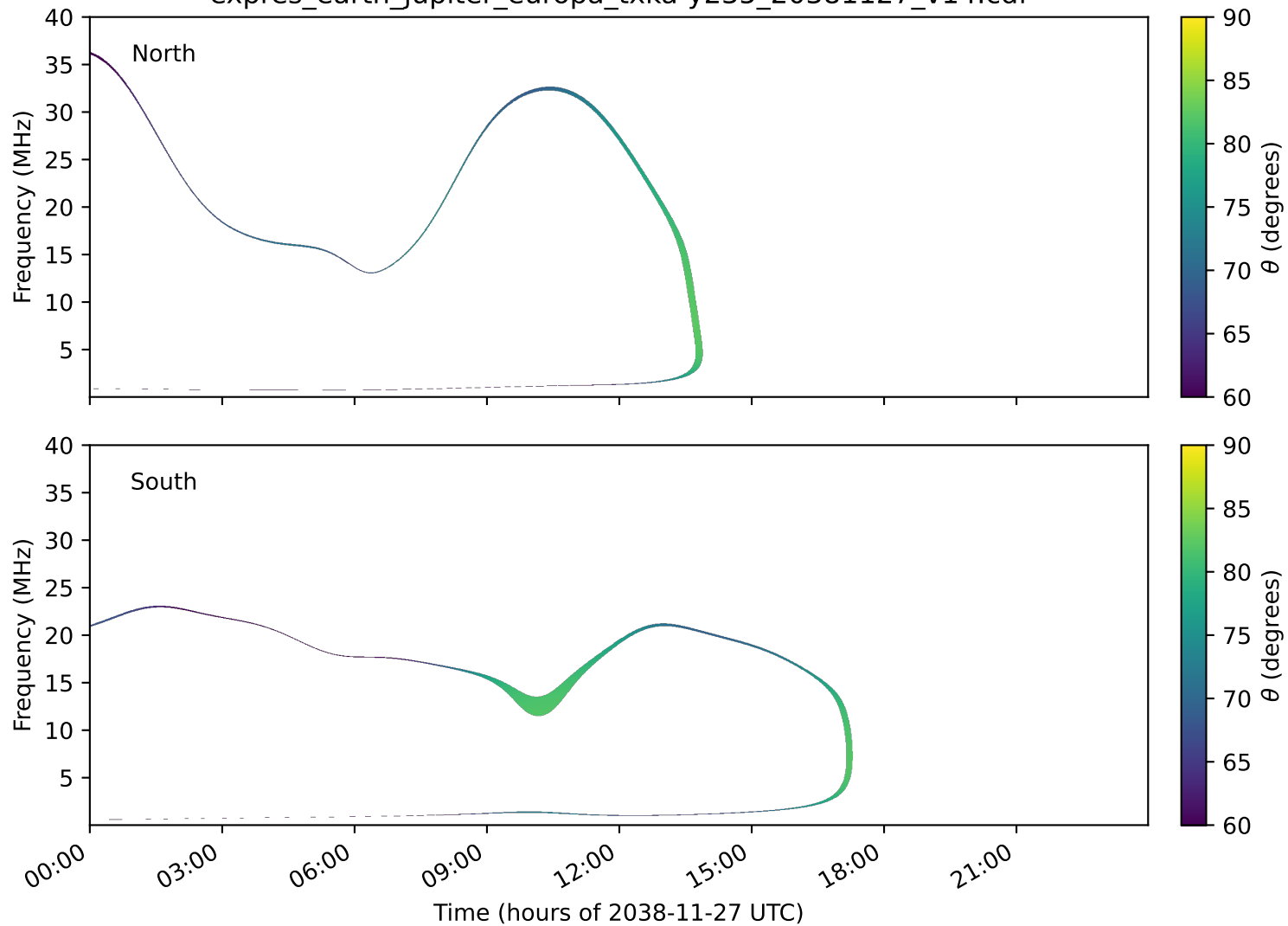
expres_earth_jupiter_europa_txka-y235_20381127_v14.cdf
