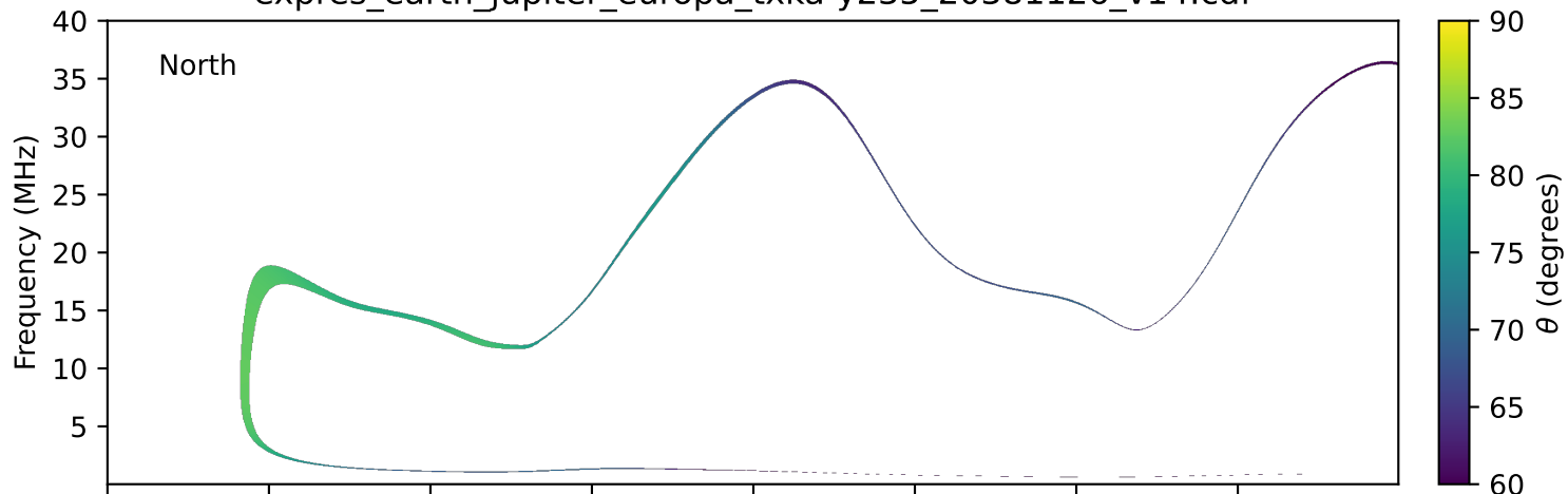
expres_earth_jupiter_europa_txka-y235_20381126_v14.cdf
