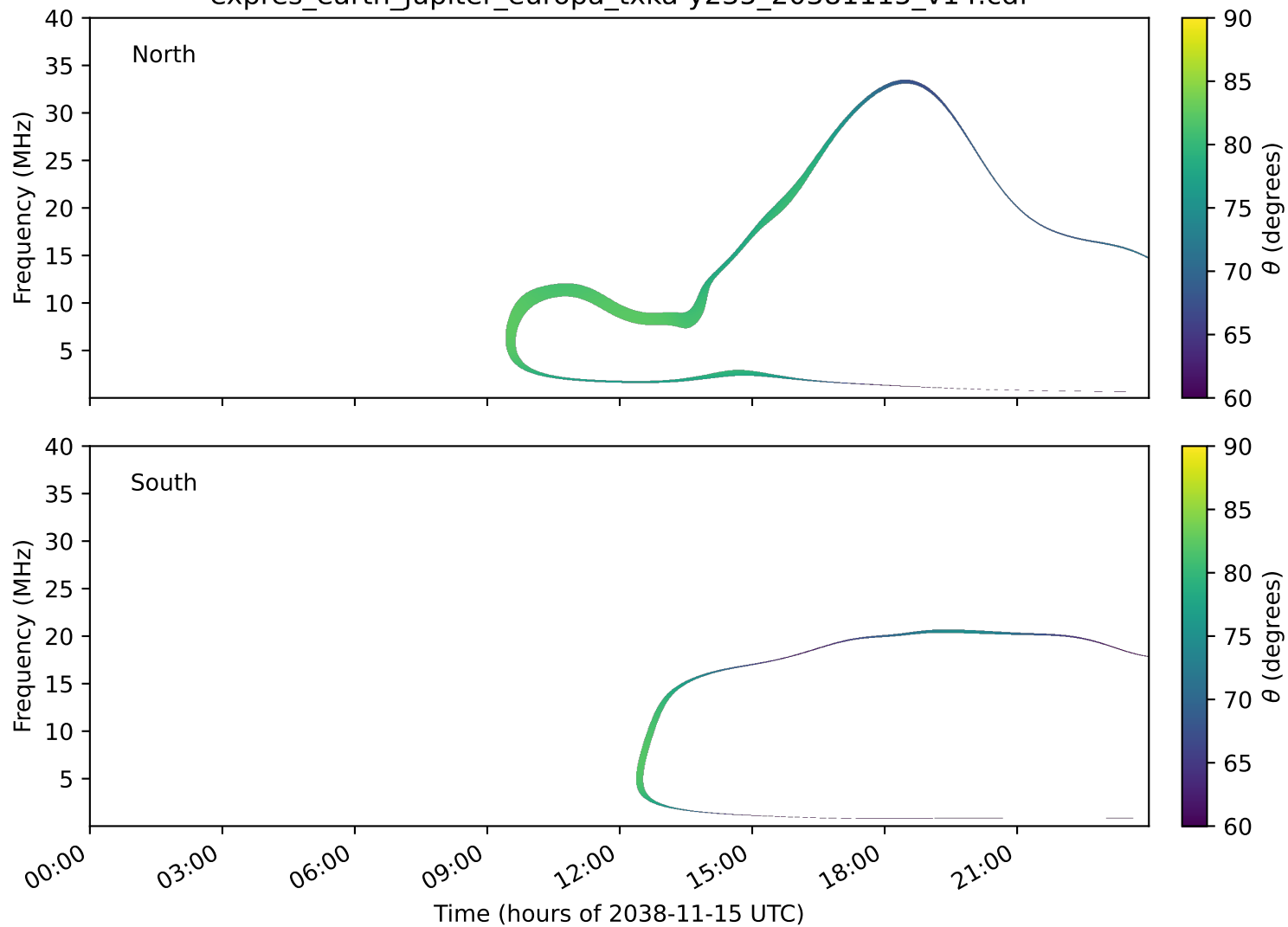
expres_earth_jupiter_europa_txka-y235_20381115_v14.cdf
