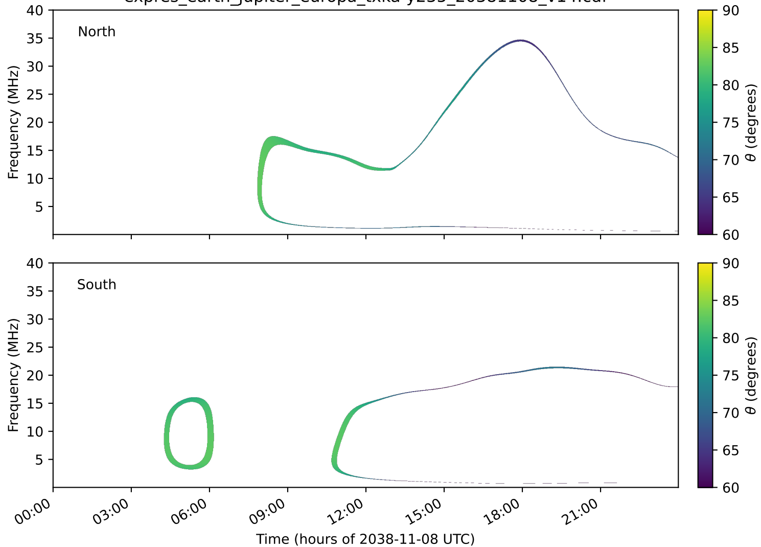
expres_earth_jupiter_europa_txka-y235_20381108_v14.cdf
