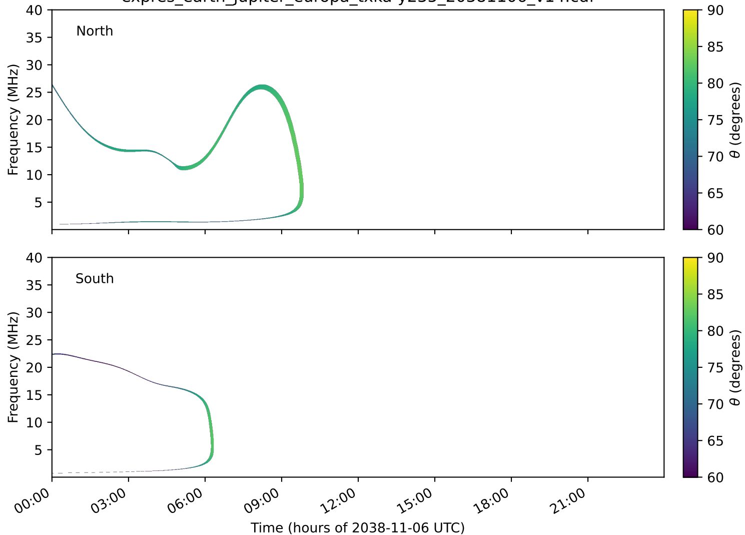
expres_earth_jupiter_europa_txka-y235_20381106_v14.cdf
