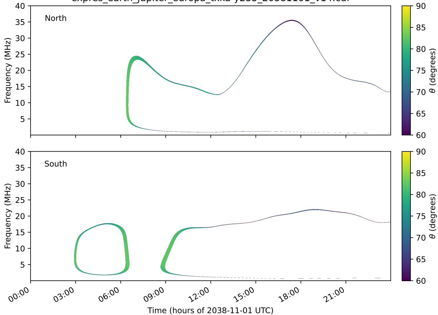
expres_earth_jupiter_europa_txka-y235_20381101_v14.cdf
