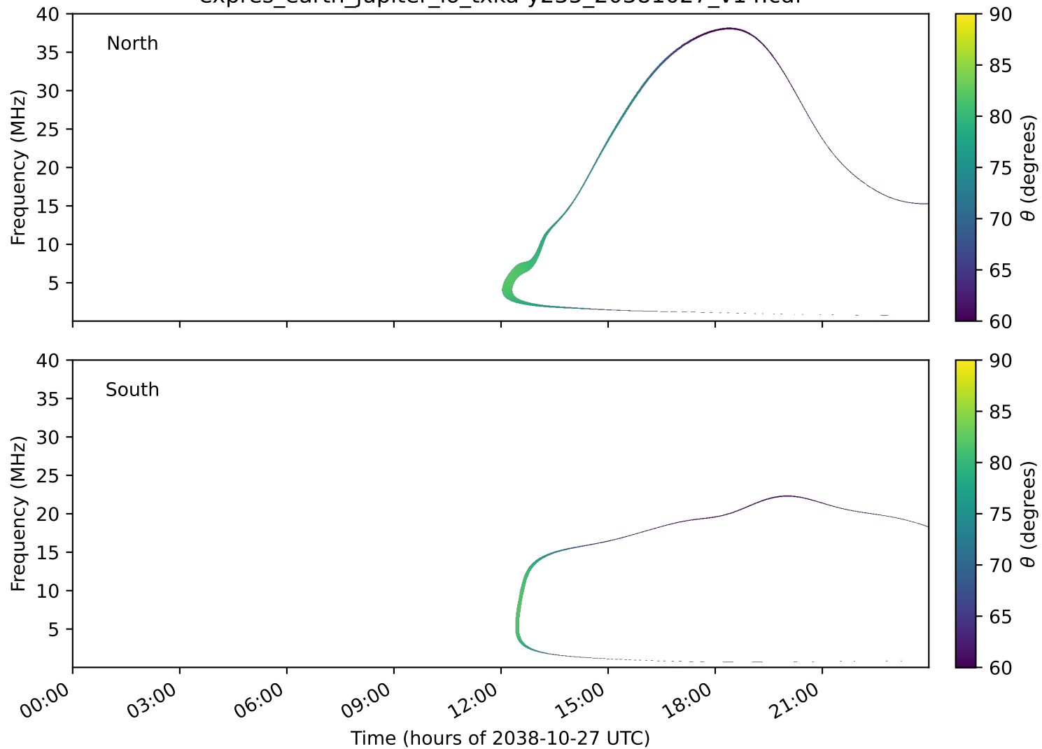
expres_earth_jupiter_io_txka-y235_20381027_v14.cdf
