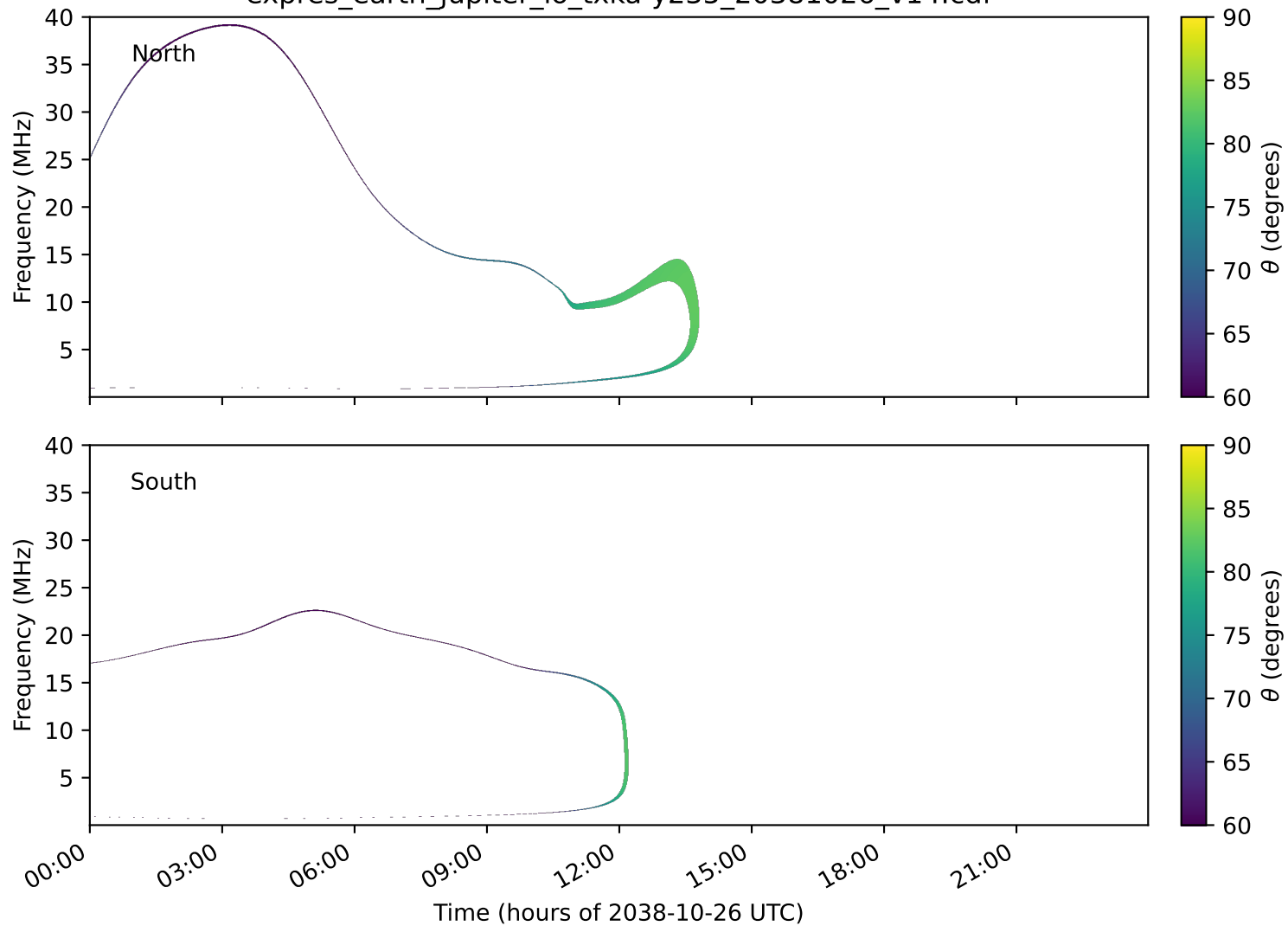
expres_earth_jupiter_io_txka-y235_20381026_v14.cdf
