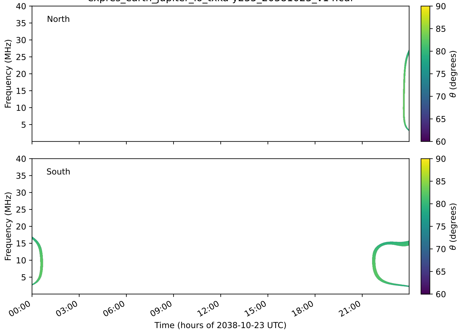
expres_earth_jupiter_io_txka-y235_20381023_v14.cdf
