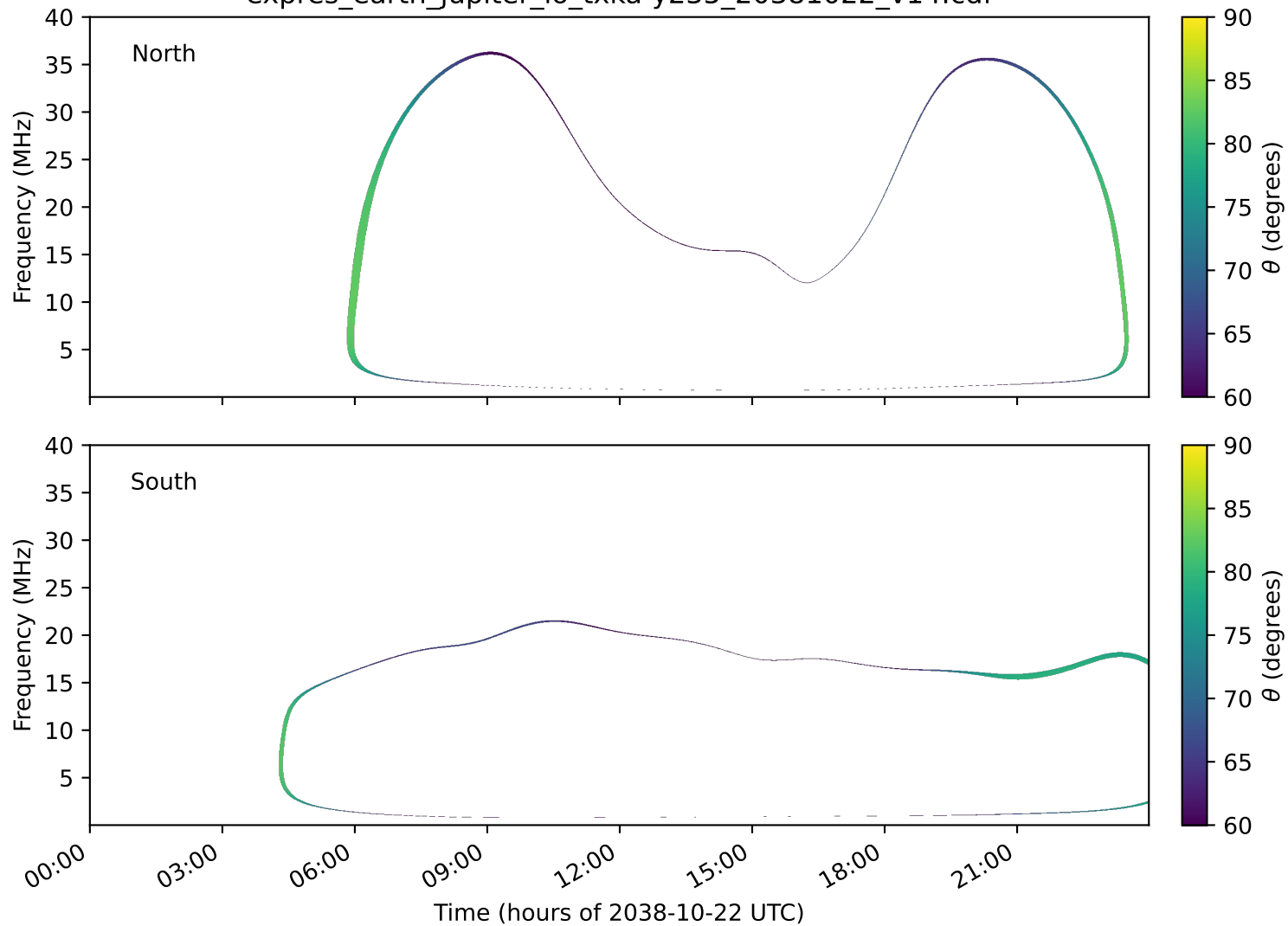
expres_earth_jupiter_io_txka-y235_20381022_v14.cdf
