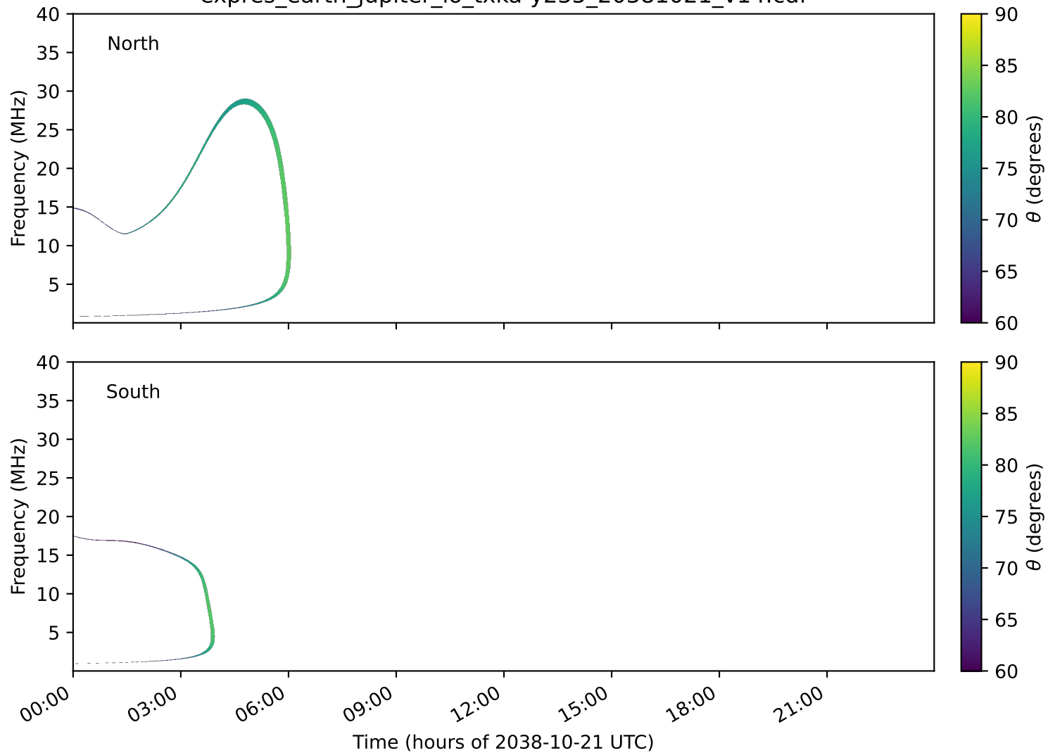
expres_earth_jupiter_io_txka-y235_20381021_v14.cdf
