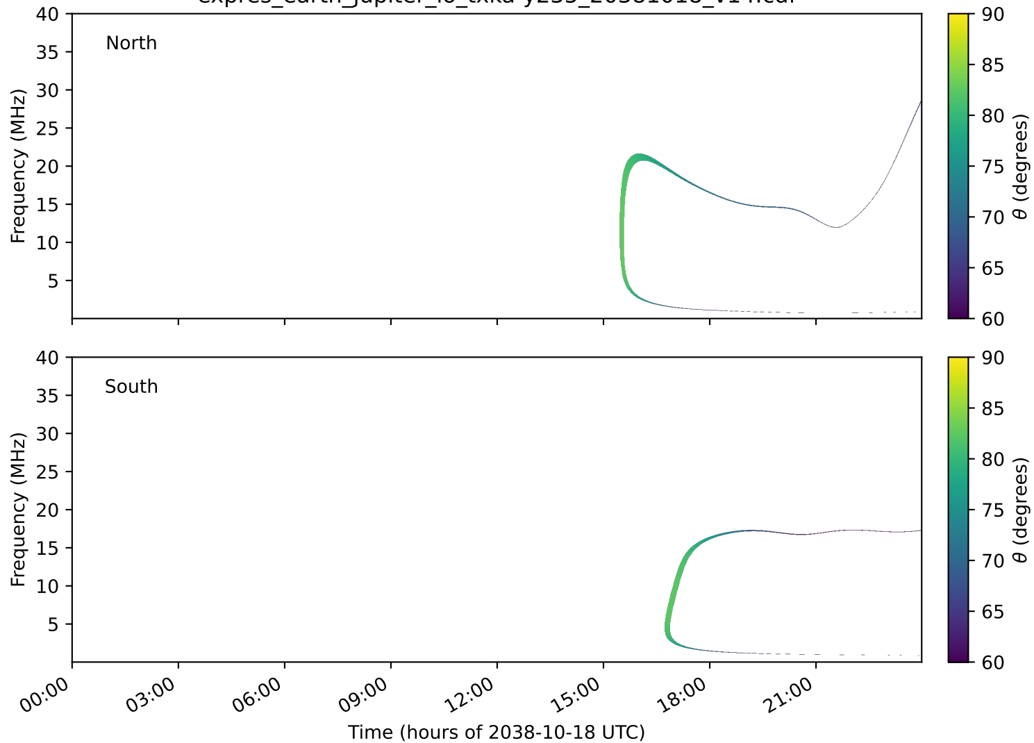
expres_earth_jupiter_io_txka-y235_20381018_v14.cdf
