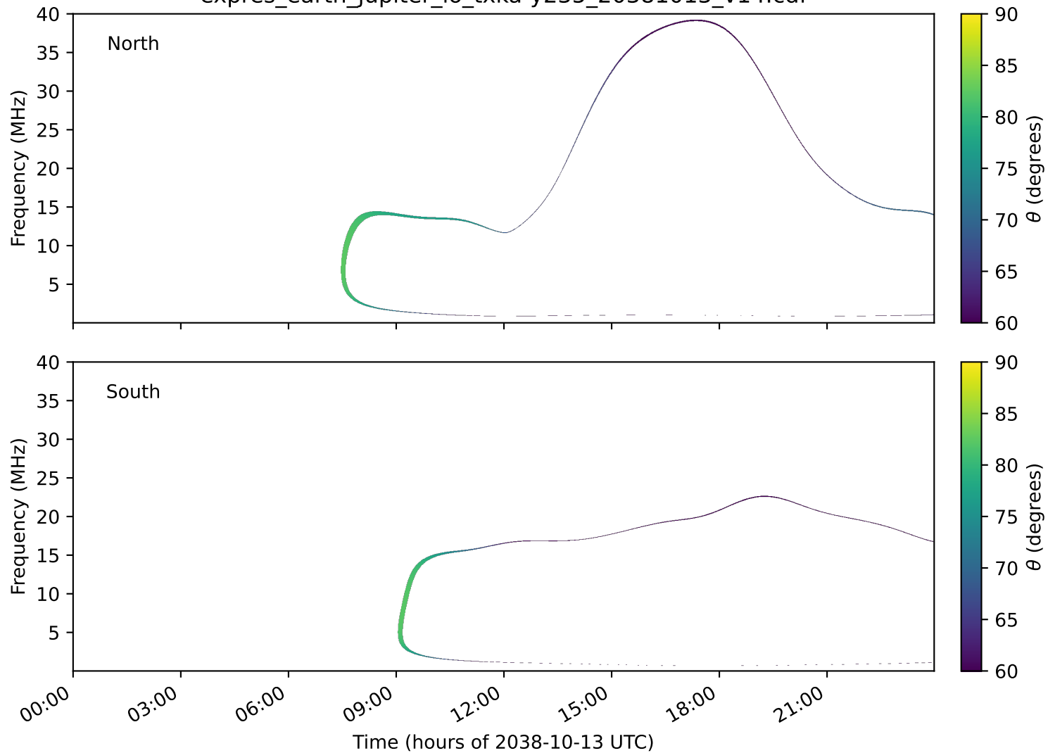
expres_earth_jupiter_io_txka-y235_20381013_v14.cdf
