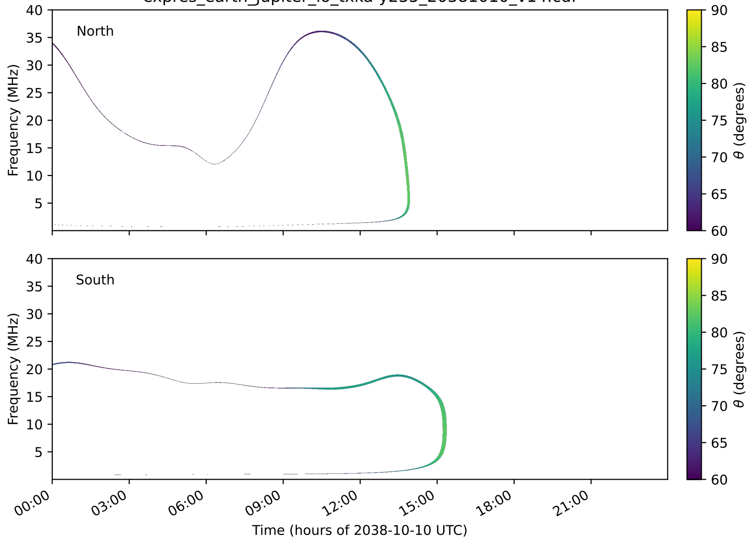
expres_earth_jupiter_io_txka-y235_20381010_v14.cdf
