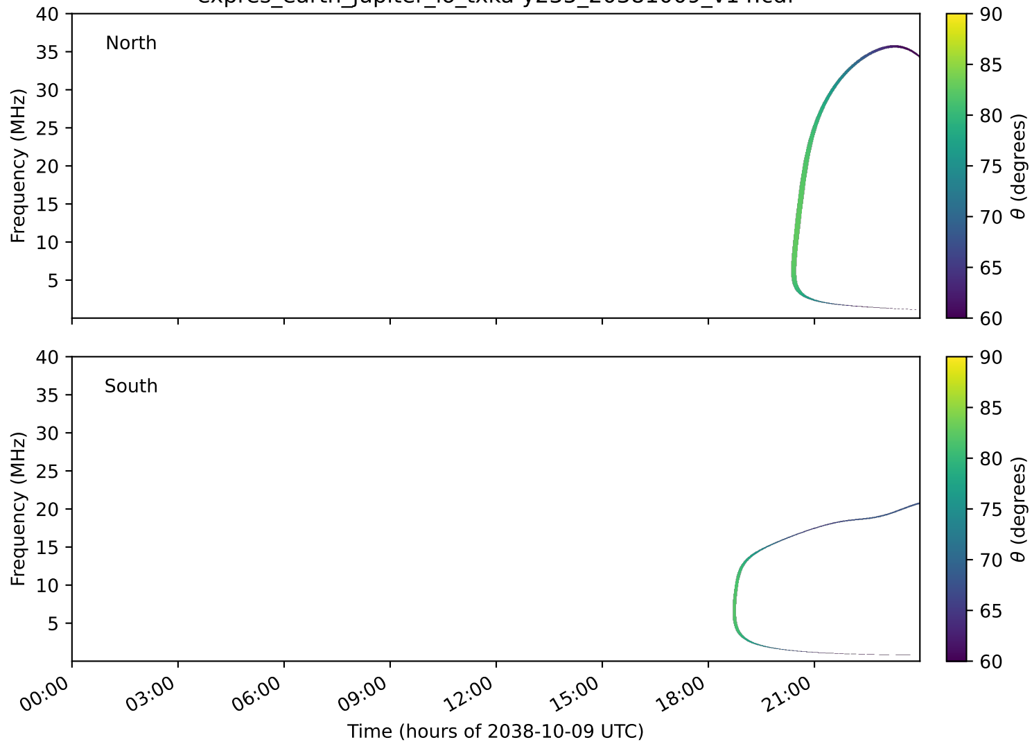
expres_earth_jupiter_io_txka-y235_20381009_v14.cdf
